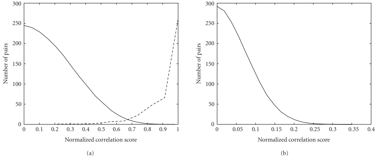
FIGURE 11: Histograms of the difference of the hash functions with 900 speech records: (a) hashes of the different objects (solid line) and those of the attacked versions of the same object (dashed line); (b) hashes obtained from the same object with different keys.
