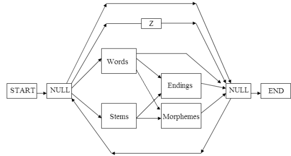
Figure 3: Combined model
