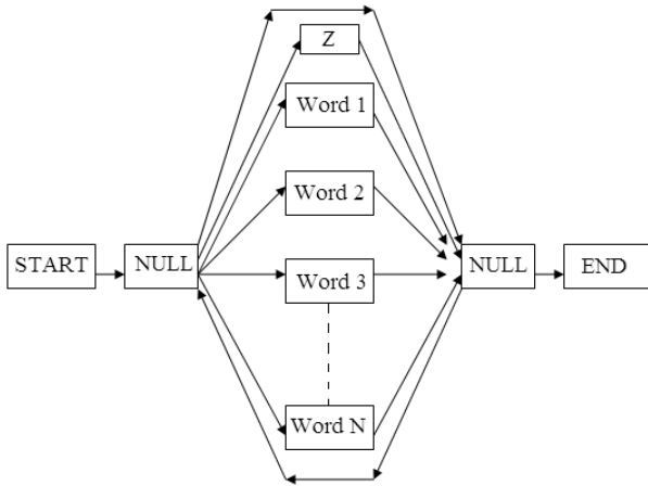
Figure 1: Word-based model
