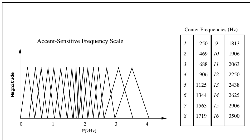
Figure 11: A new sampling scheme for the filter banks which is more sensitive to accent characteristics.
