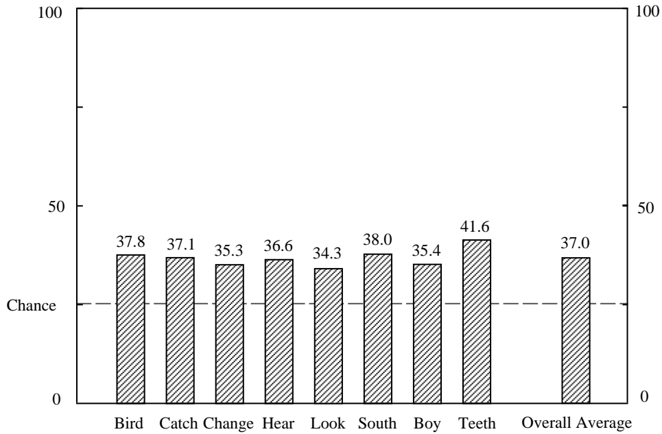
Accent Classification Using Average Voicing Duration
